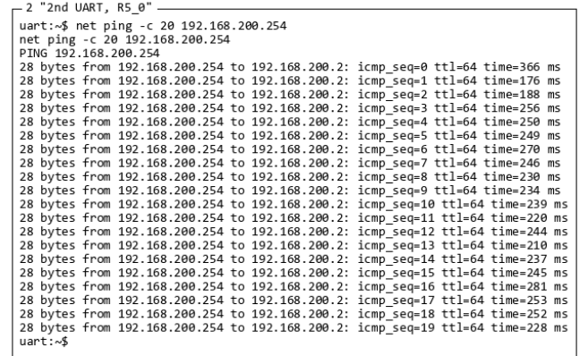
Fig. 5. Executing a ping from the Zephyr remote back to the Linux host
